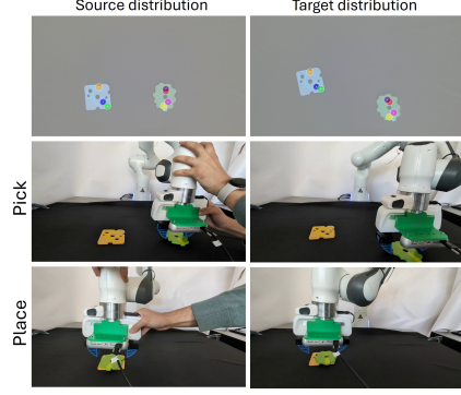
Figure 5: Food Stacking Task. The single demonstration is shown on the left, and the corresponding motion generalization on the right. Source and target keypoints are automatically extracted using DINO features correspondences [19], with their 3D positions estimated from a stereoscopic depth map. A kinesthetic demonstration is performed by the user, and a transportation policy is used to generalize the motion across different object configurations.
