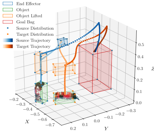
Figure 6: The left picture depicts the setup used for performing the experiments. The right picture shows the source keypoints and trajectory as well as the target ones for one of the tests. It can be observed how the source trajectory gets deformed and successfully places the object inside the bag.
