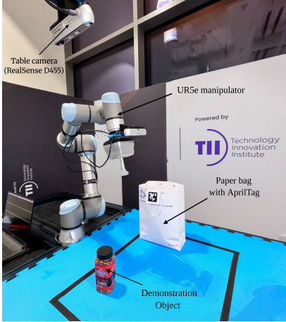
Figure 6: The left picture depicts the setup used for performing the experiments. The right picture shows the source keypoints and trajectory as well as the target ones for one of the tests. It can be observed how the source trajectory gets deformed and successfully places the object inside the bag.
